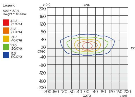
Isolux Diagram
